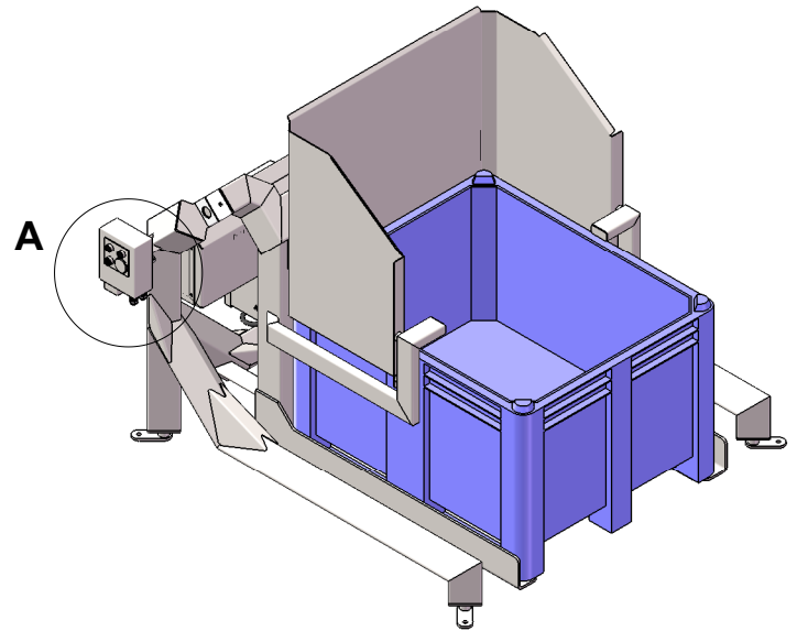
Bolted base version
